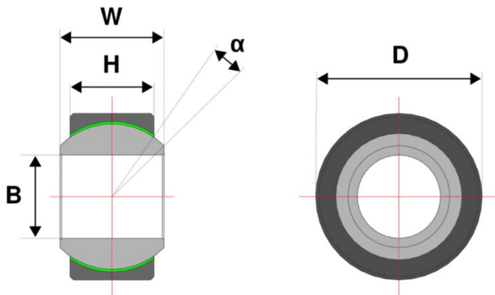
spherical bearing
